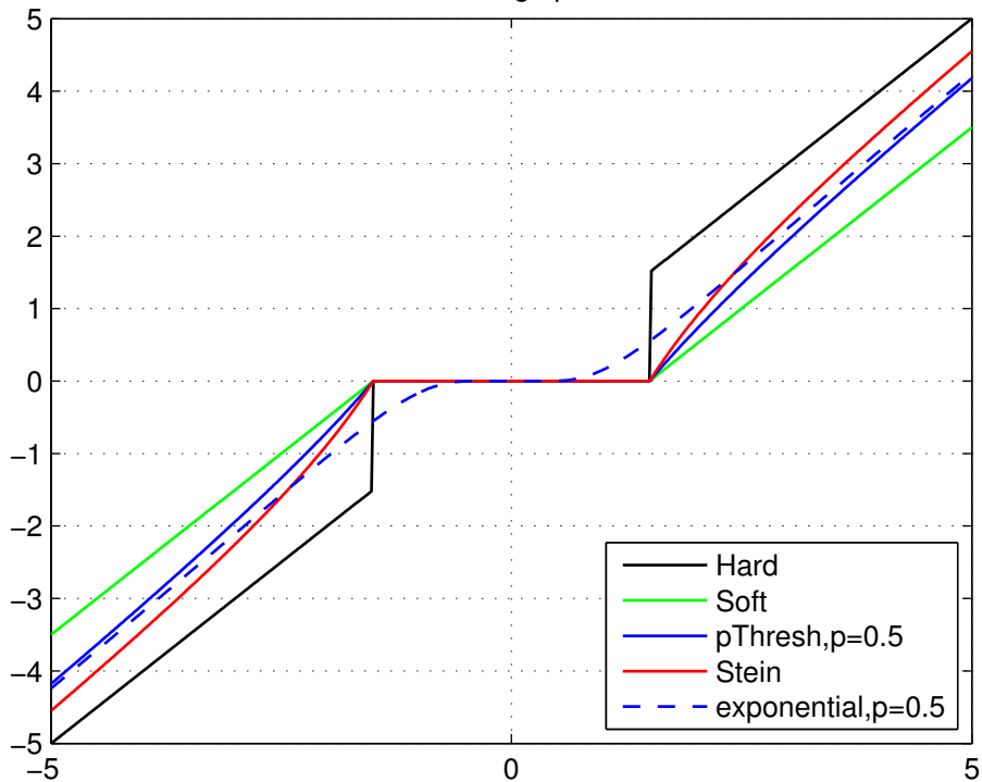
Thresholding operators
