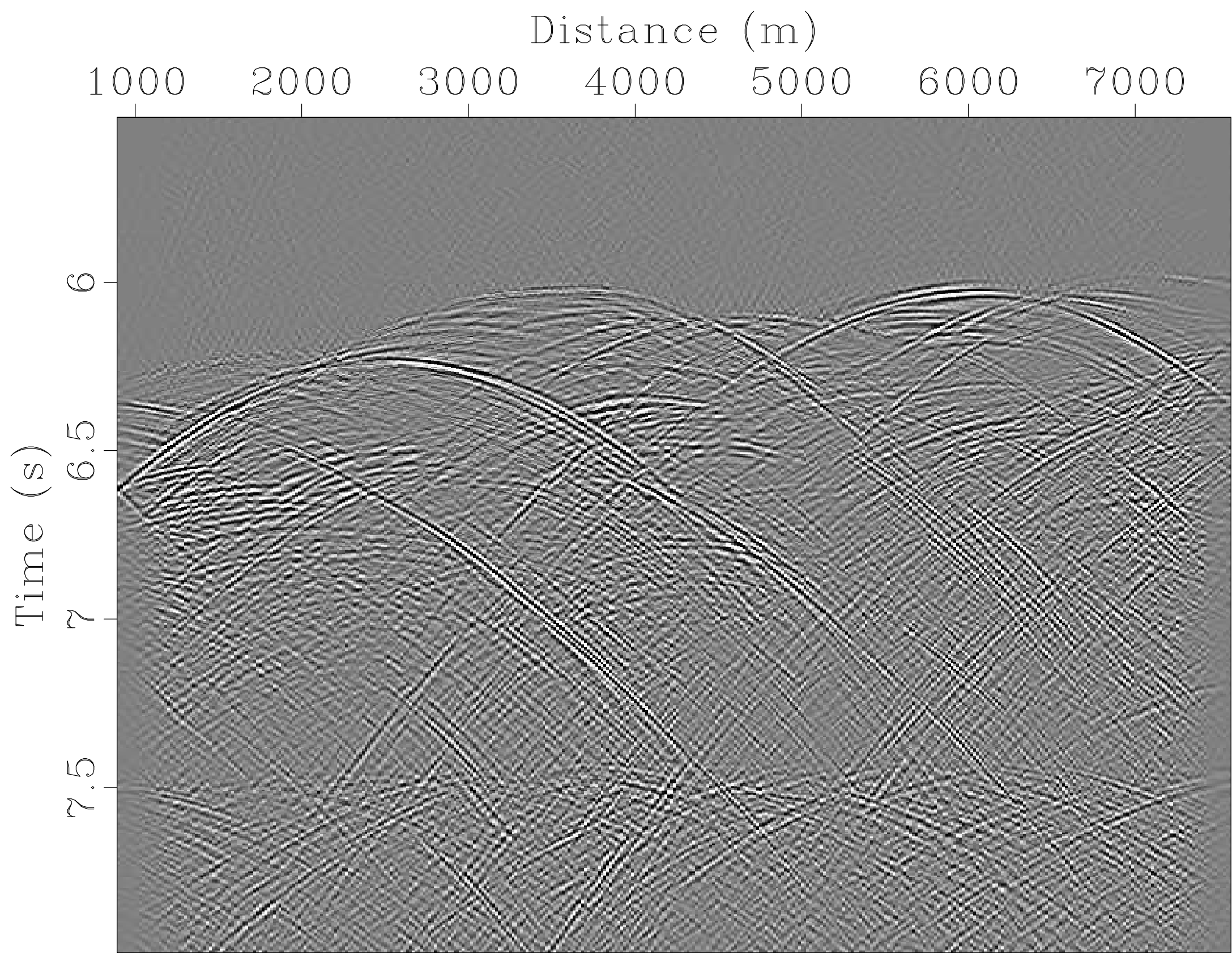
Diffraction Data
