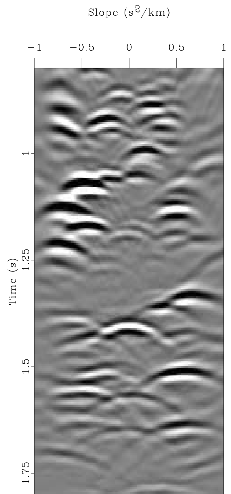
Slope Gather ( x=2.32 km, v=3.9 km/s)
