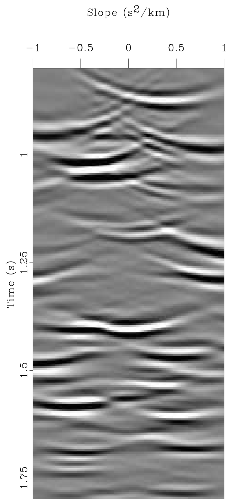
Slope Gather ( x=2.32 km, v=2.1 km/s)
