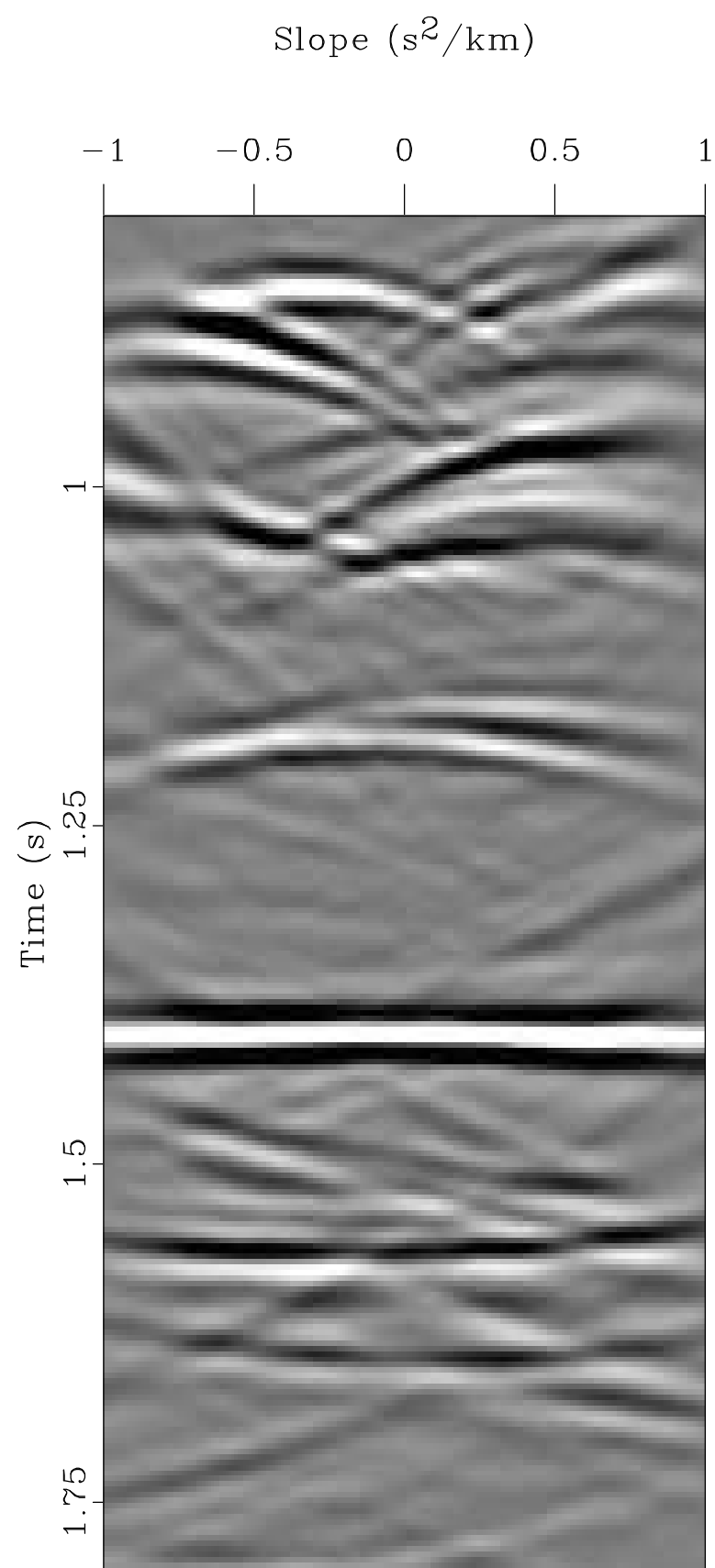
Slope Gather ( x=2.32 km, v=3 km/s)
