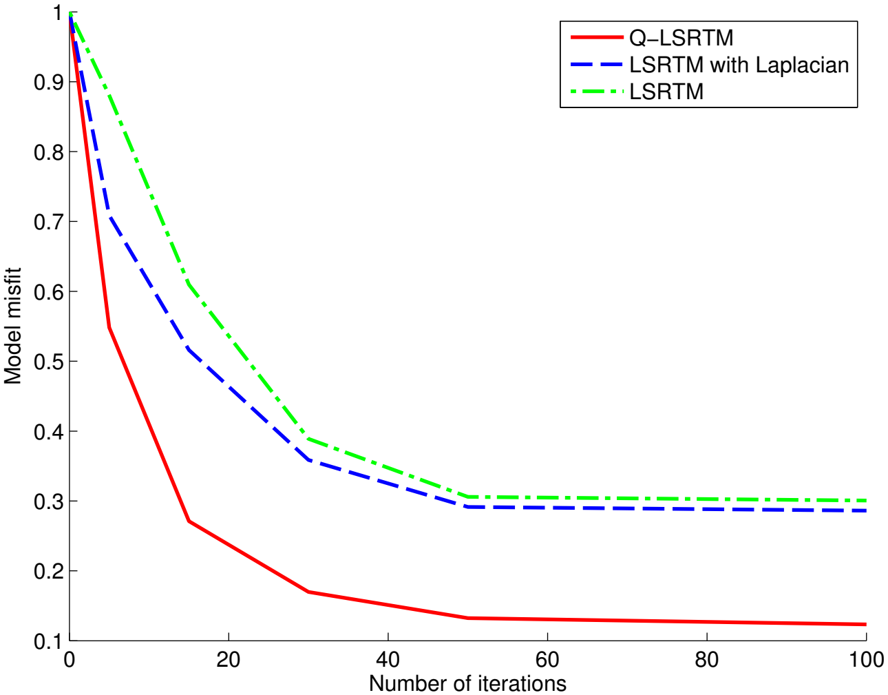
Convergence curve
