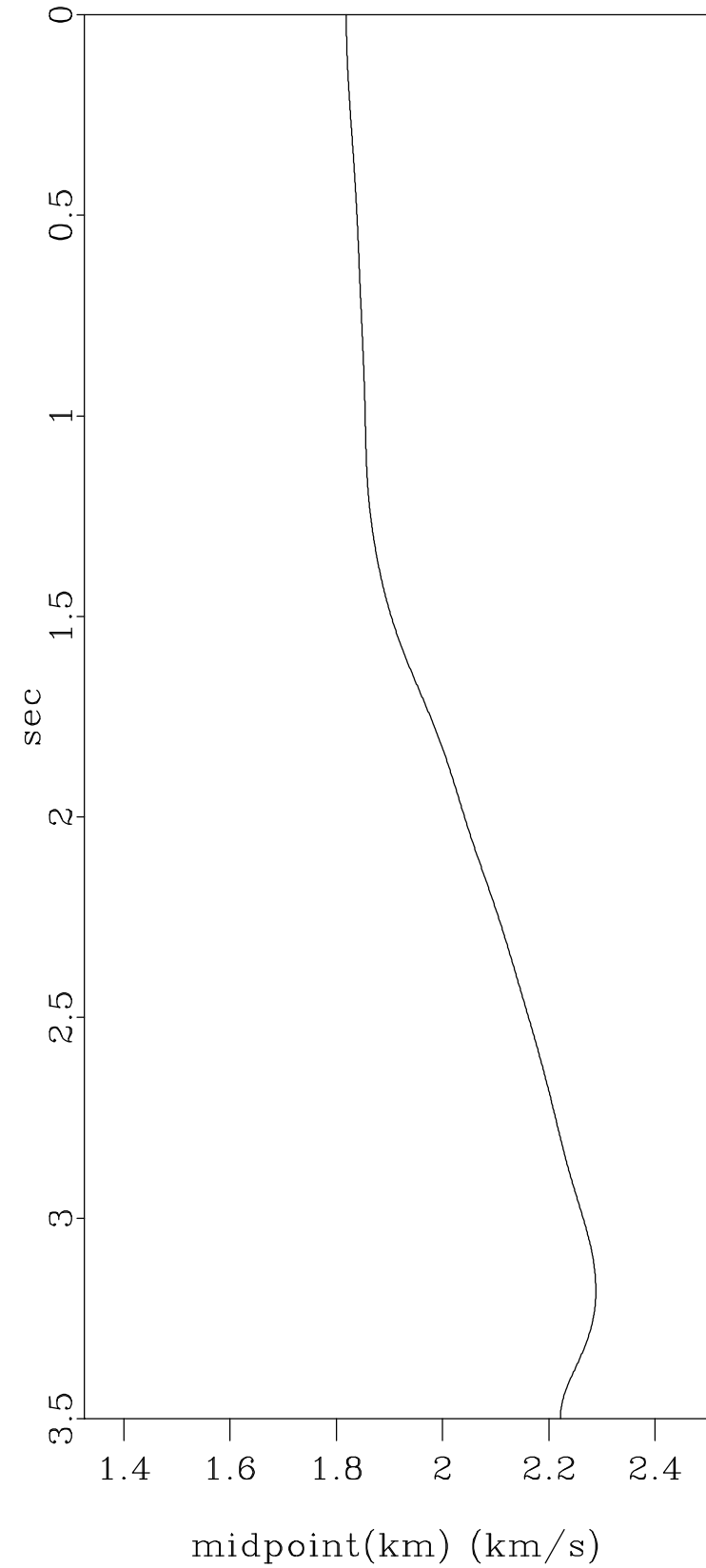
epsilon=0.5
