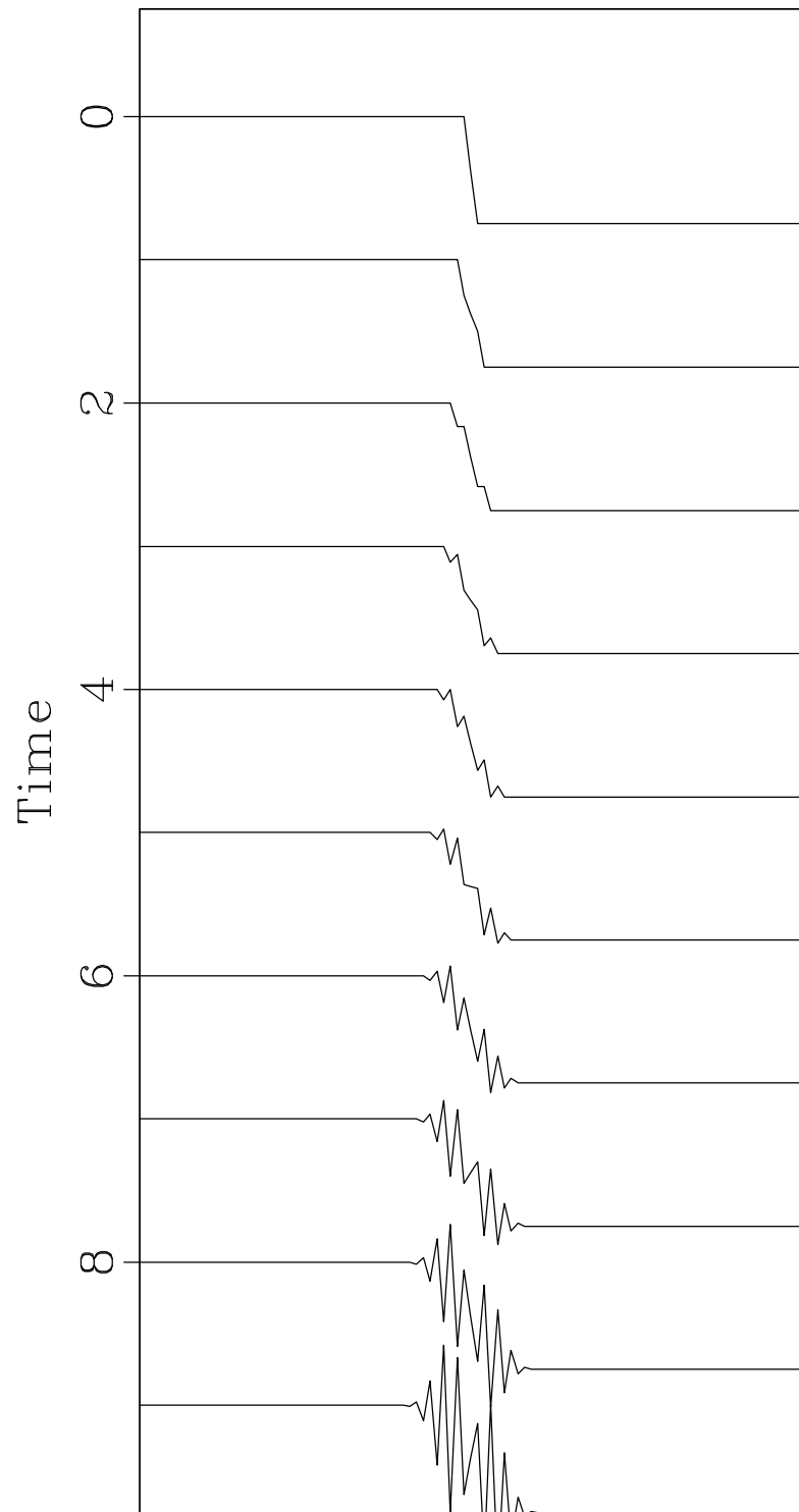
Explicit, a=4/3
