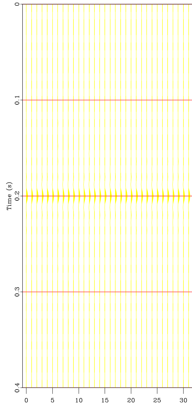
Estimated Noise
