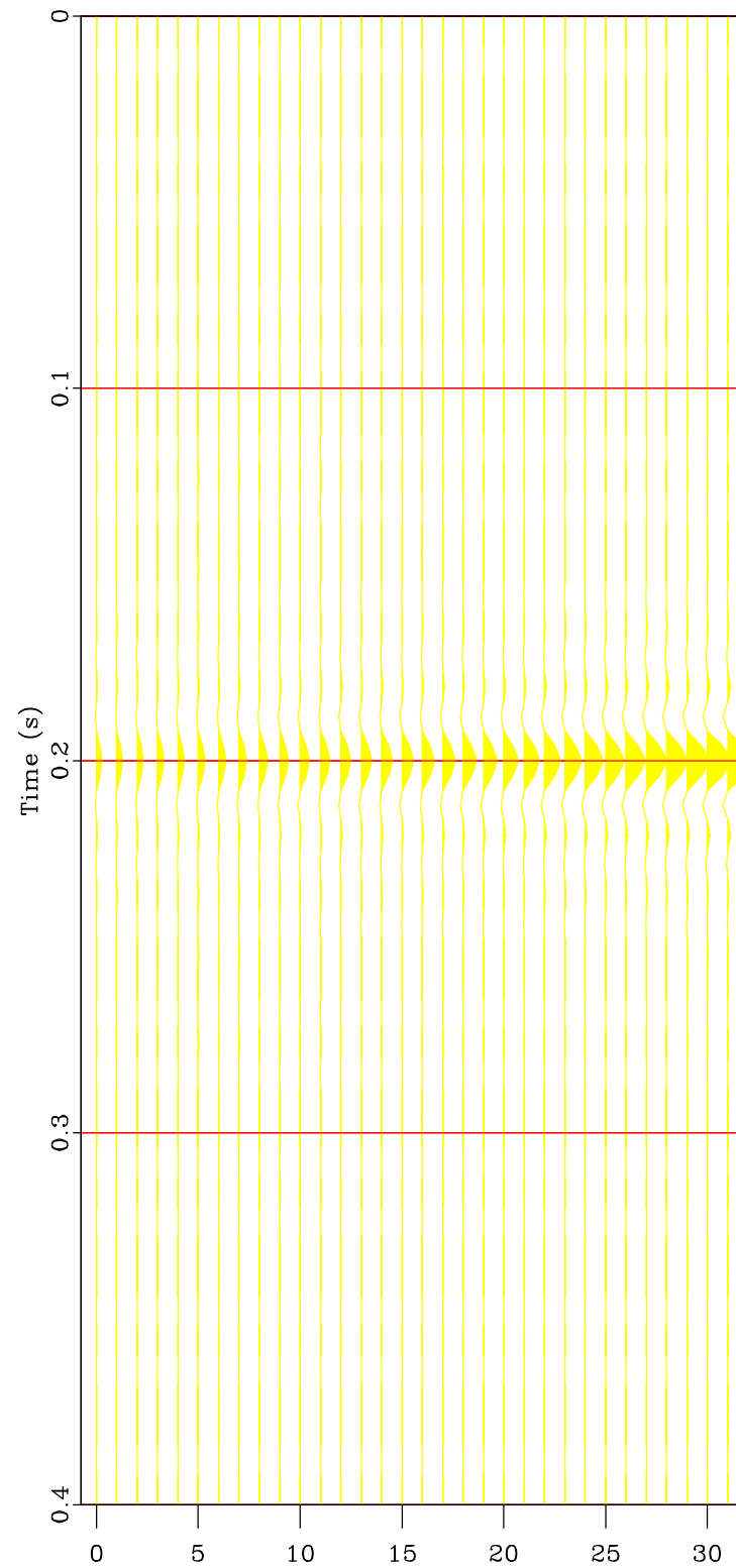
Estimated Signal
