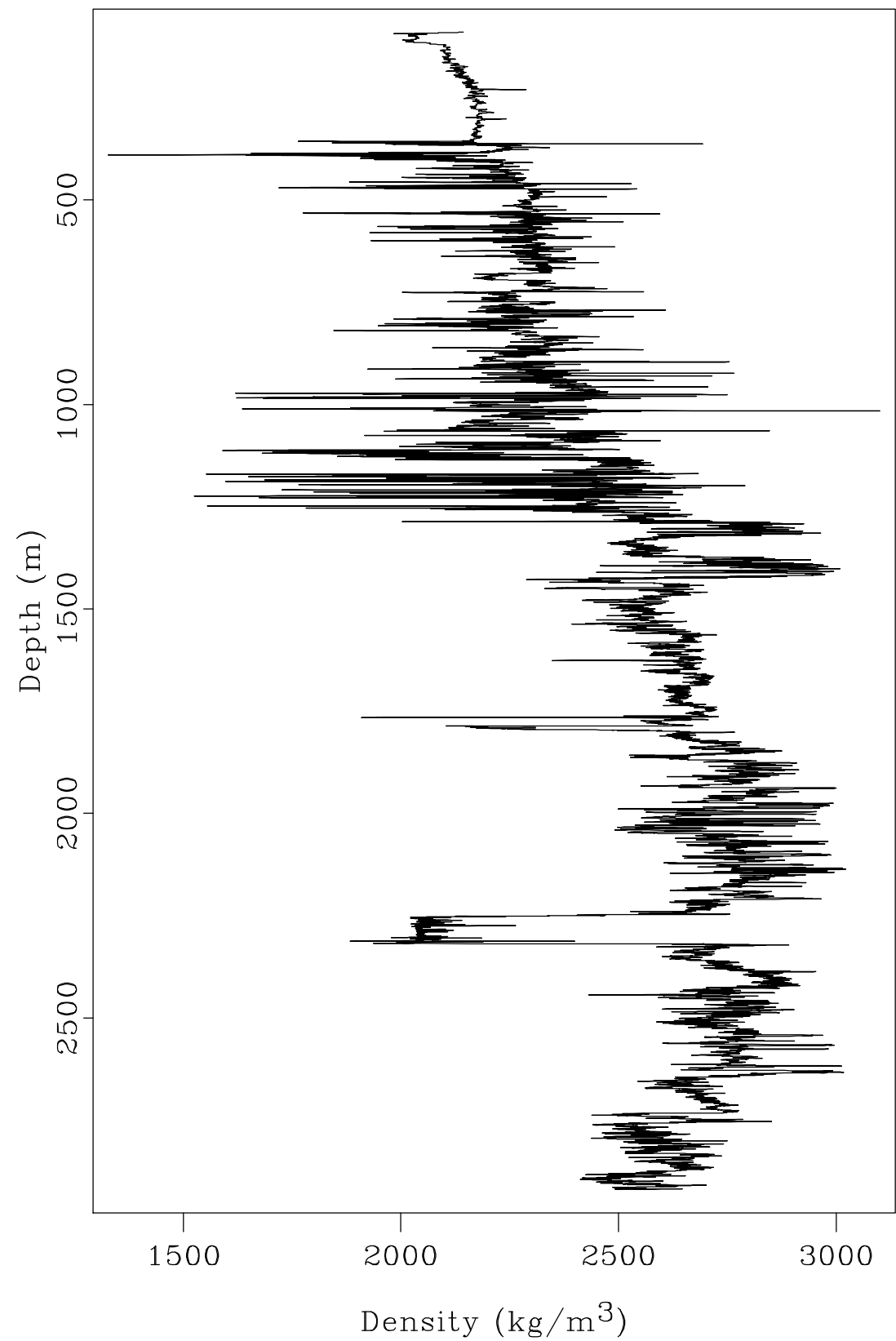
Sonic Density
