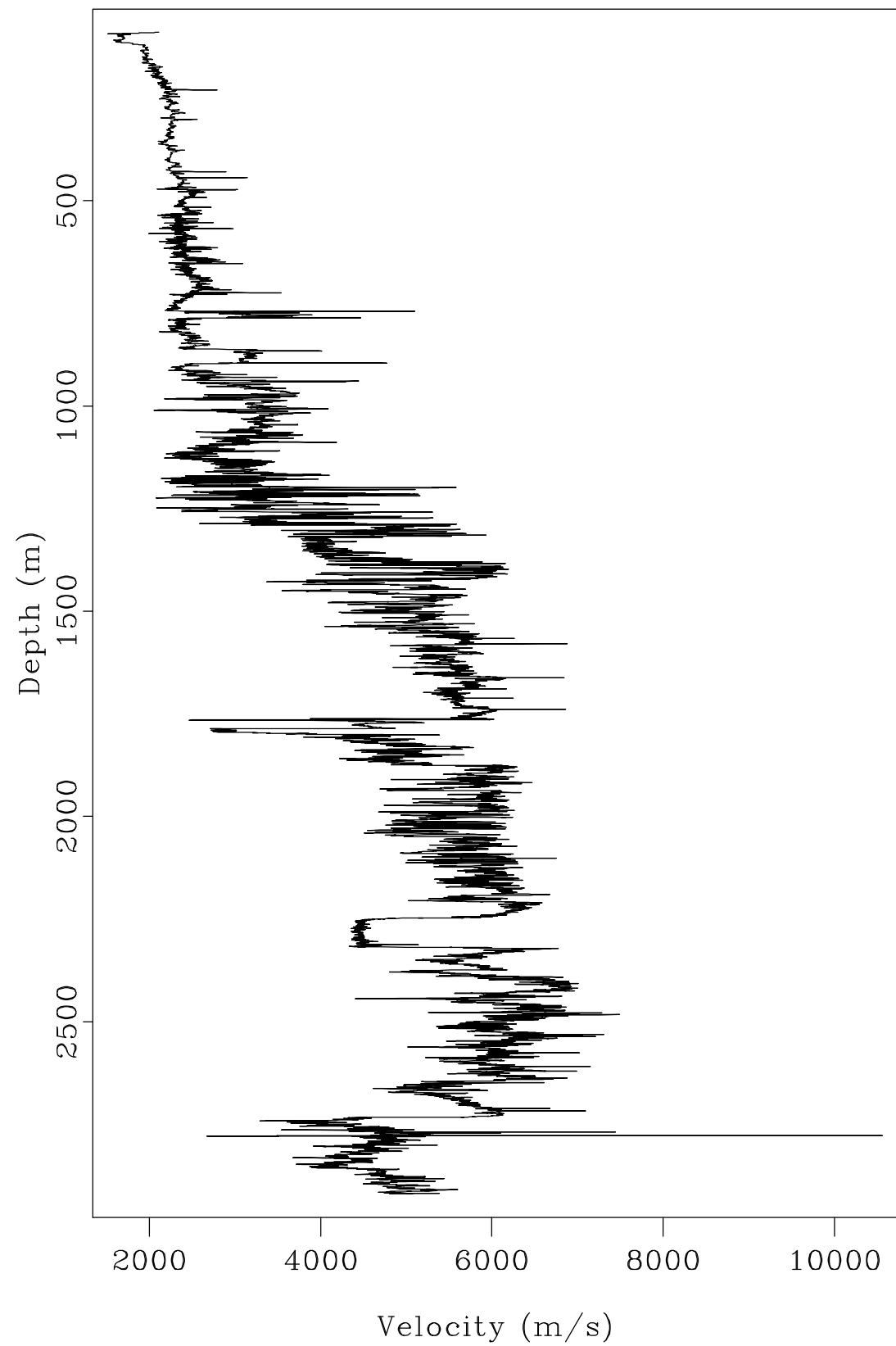
Sonic Velocity
