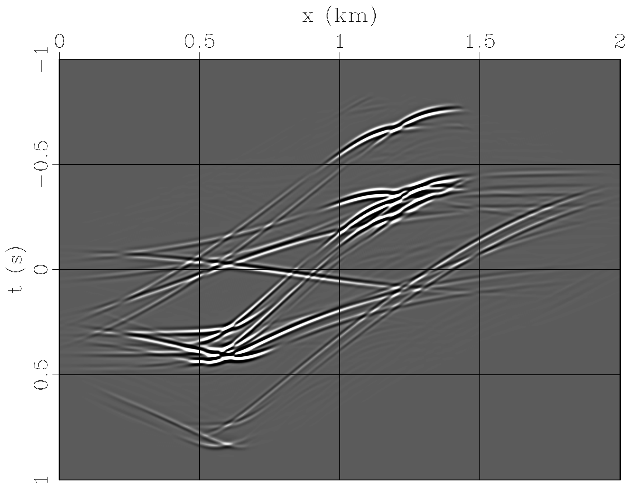
top: total integrand (w/ taper)
