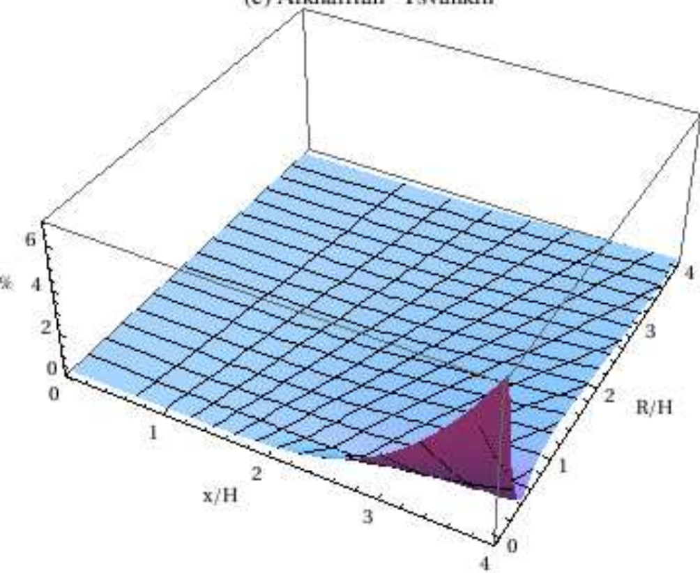
(c) Alkhalifah-Tsvankin
