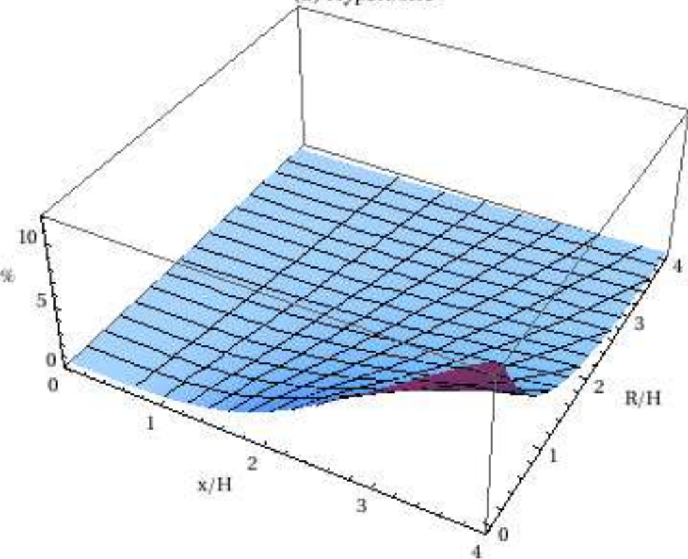
(a) Hyperbolic
