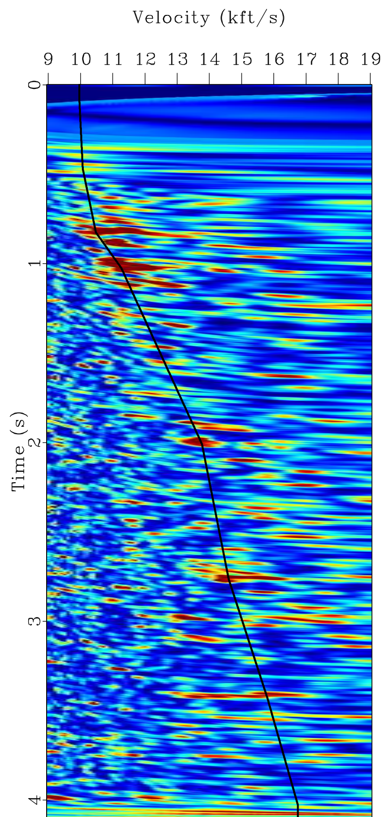
Semblance Scan
