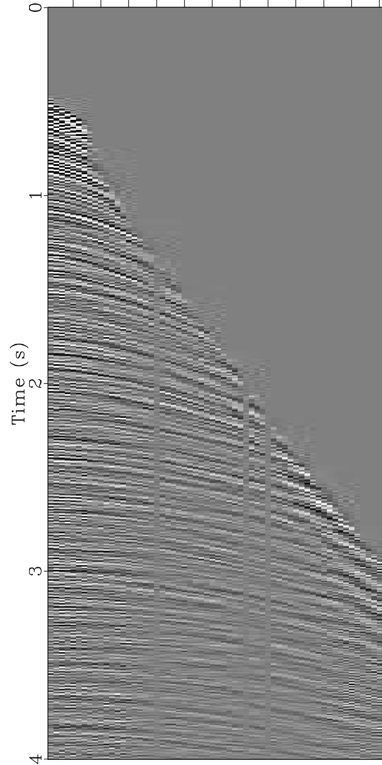
CMP gather 700
