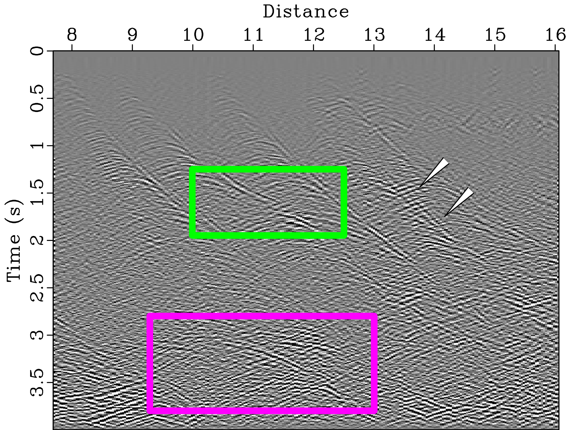
Separated diffractions by PWD
