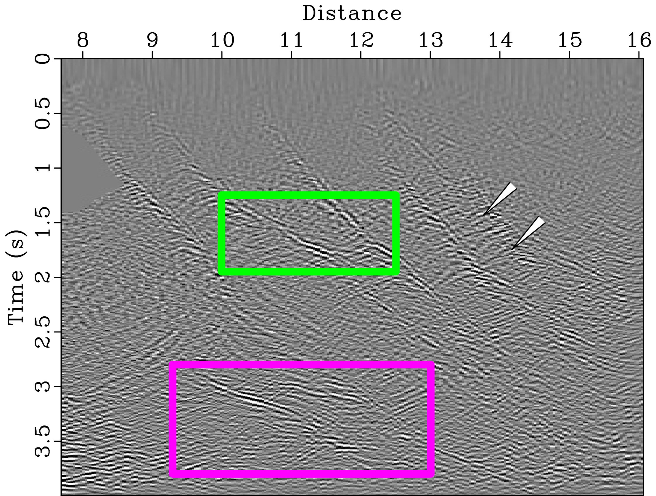
Migrated Diffractions LRRA
