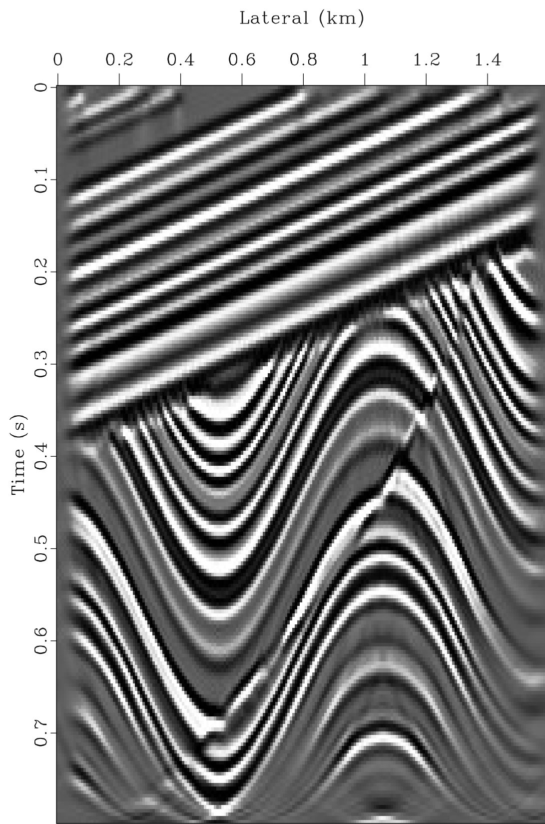
Stolt \rightarrow Velocity Continuation
