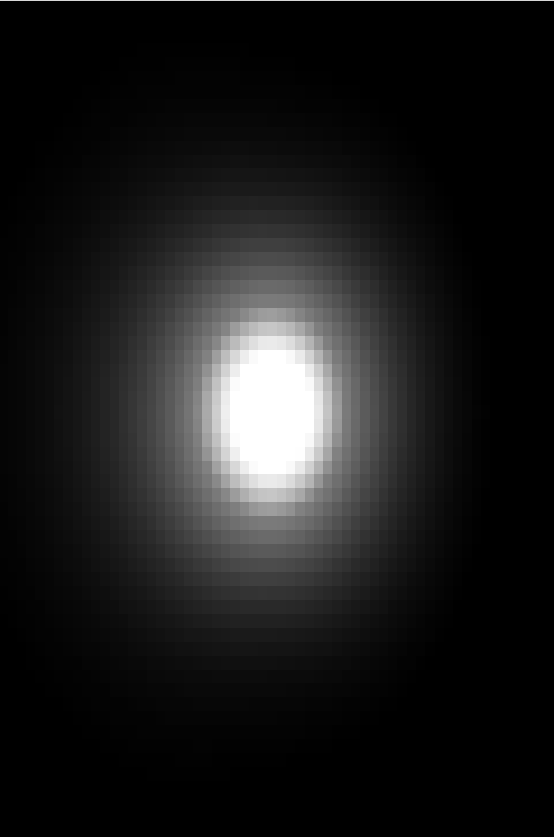
Factorization
