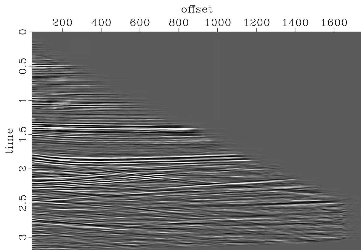
interpolated shot
