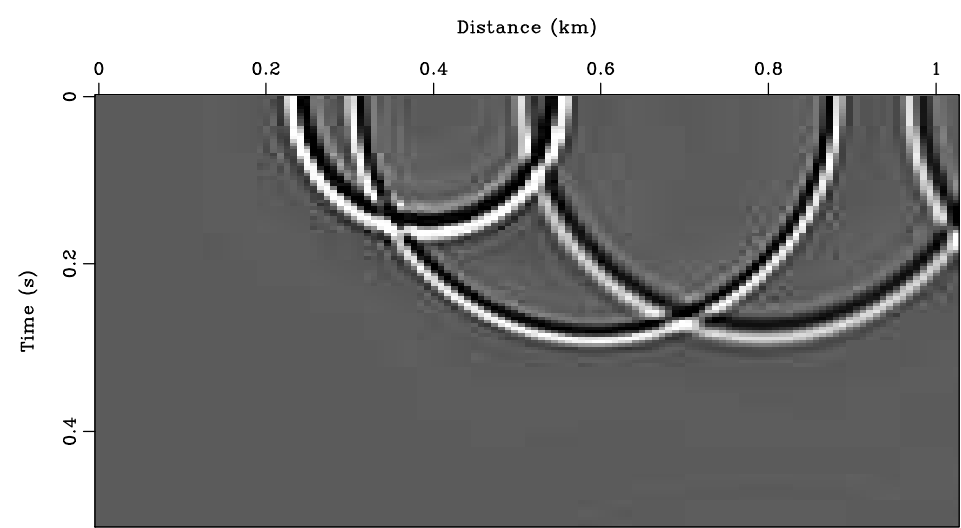
Stolt migration 8: In-line slice
