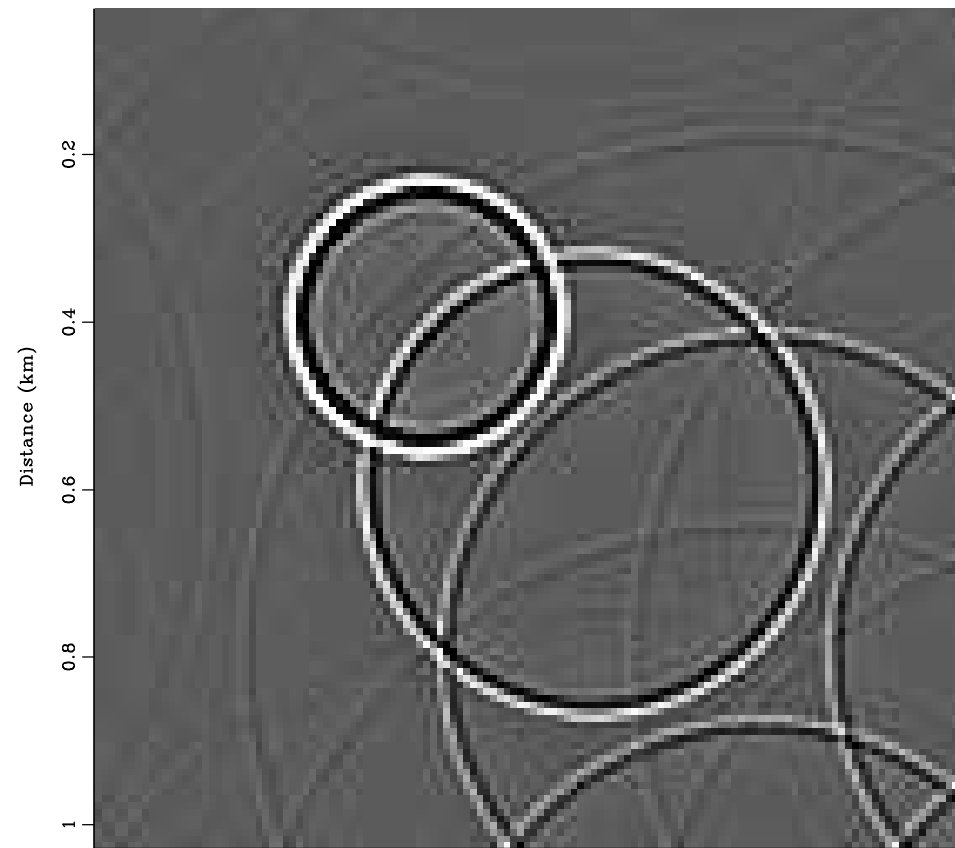
Stolt migration 2: Depth slice
