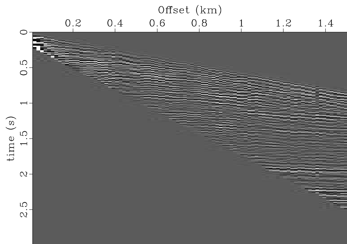
B-4 interpolation
