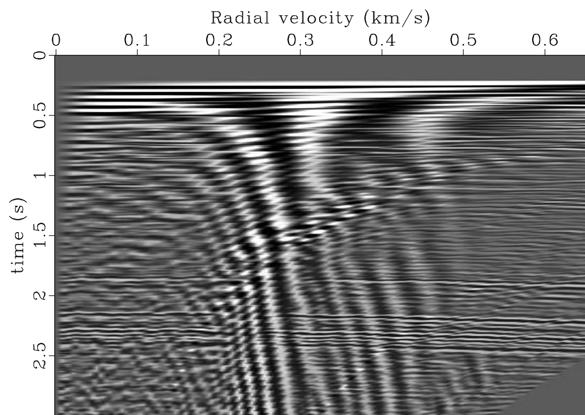
B-2 interpolation
