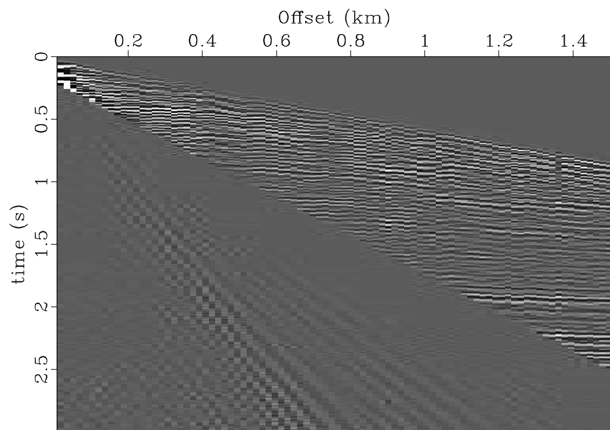
B-2 interpolation
