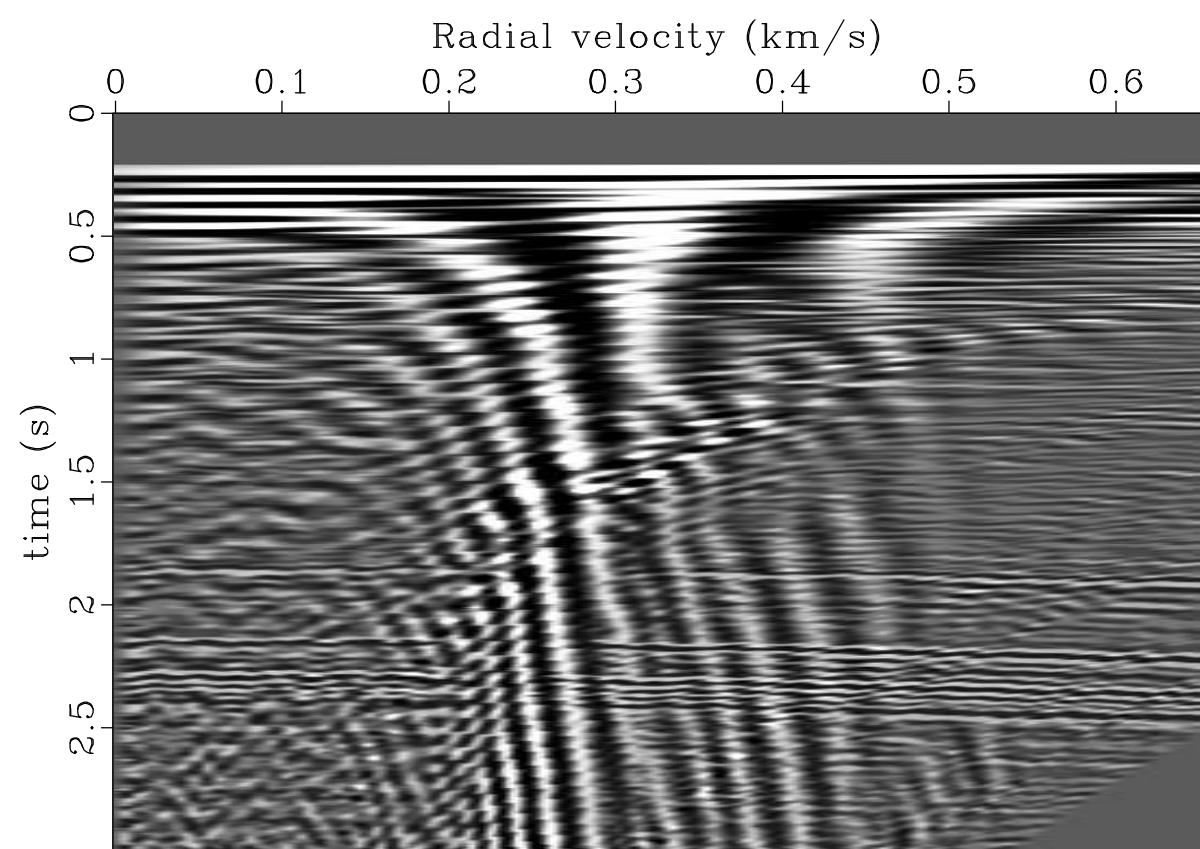
B-4 interpolation
