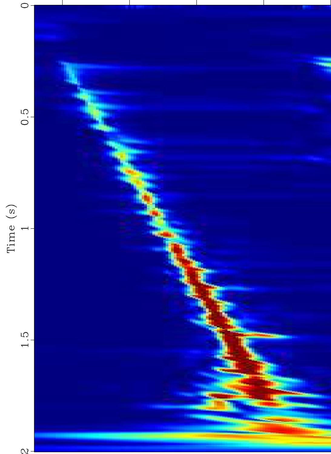
Primaries Semblance Scan
