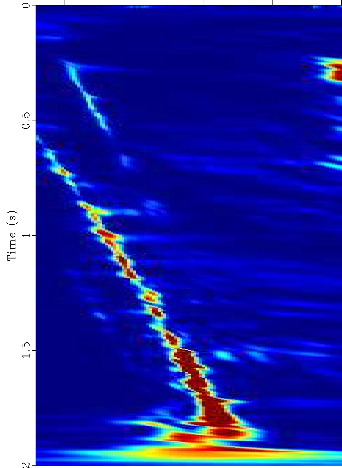
Multiples Semblance Scan
