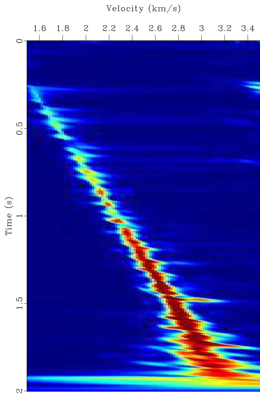
Primaries Semblance Scan
