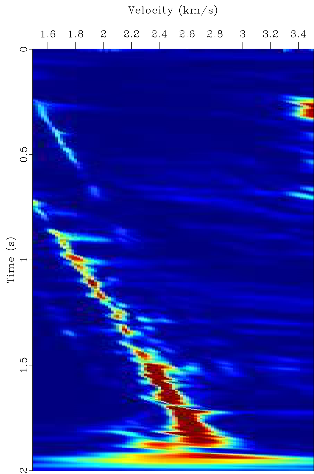
Multiples Semblance Scan
