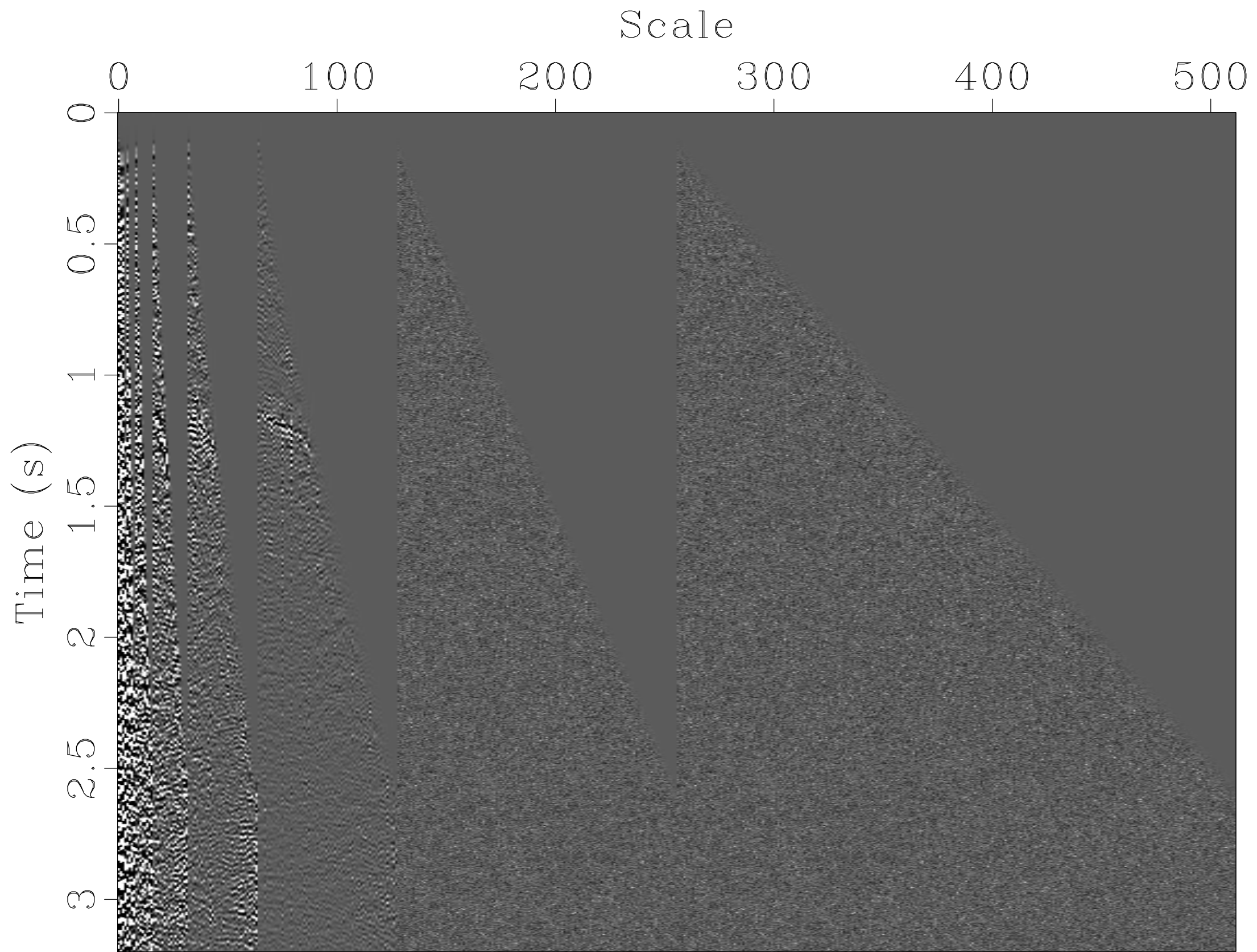
Seislet Transform
