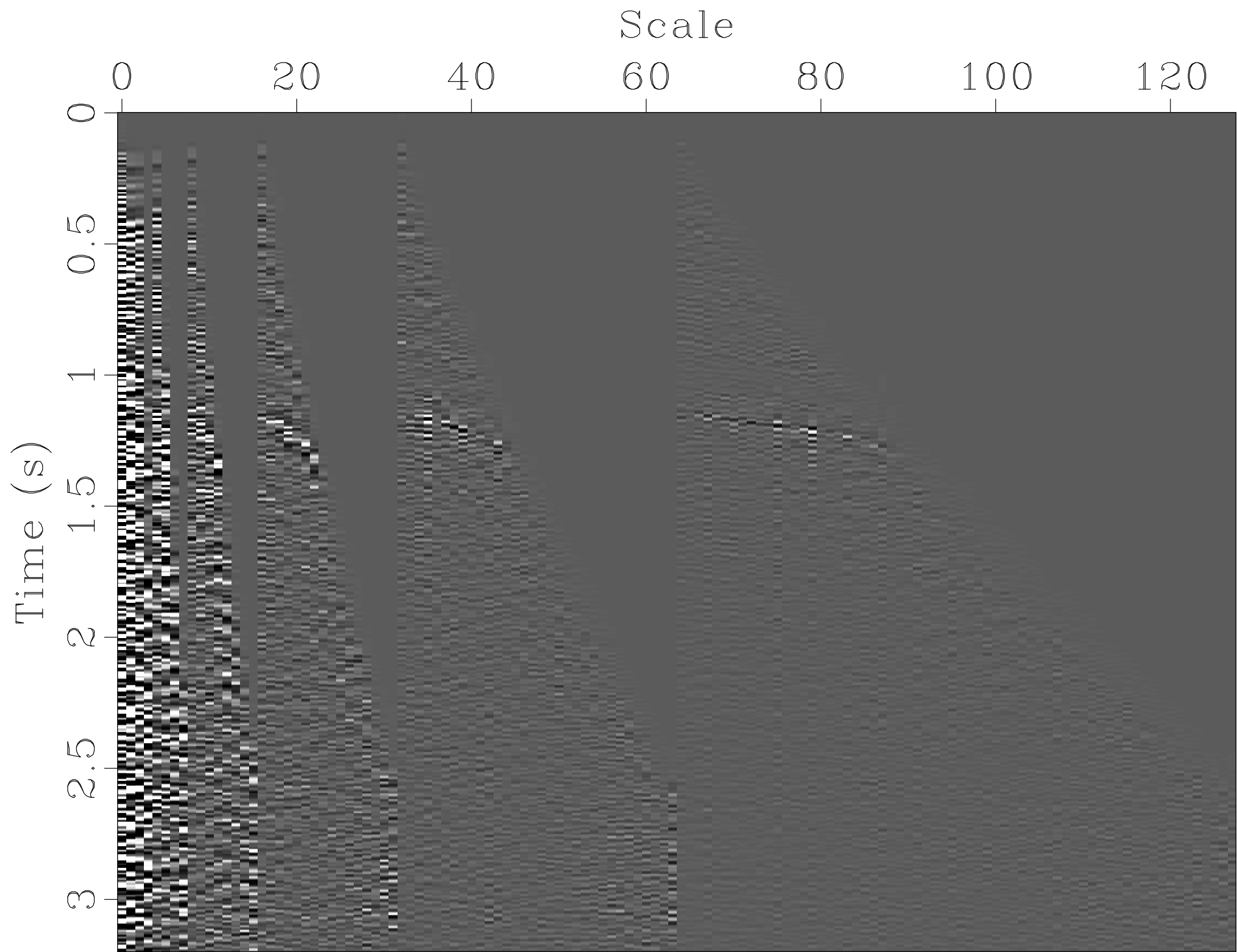
Seislet Transform
