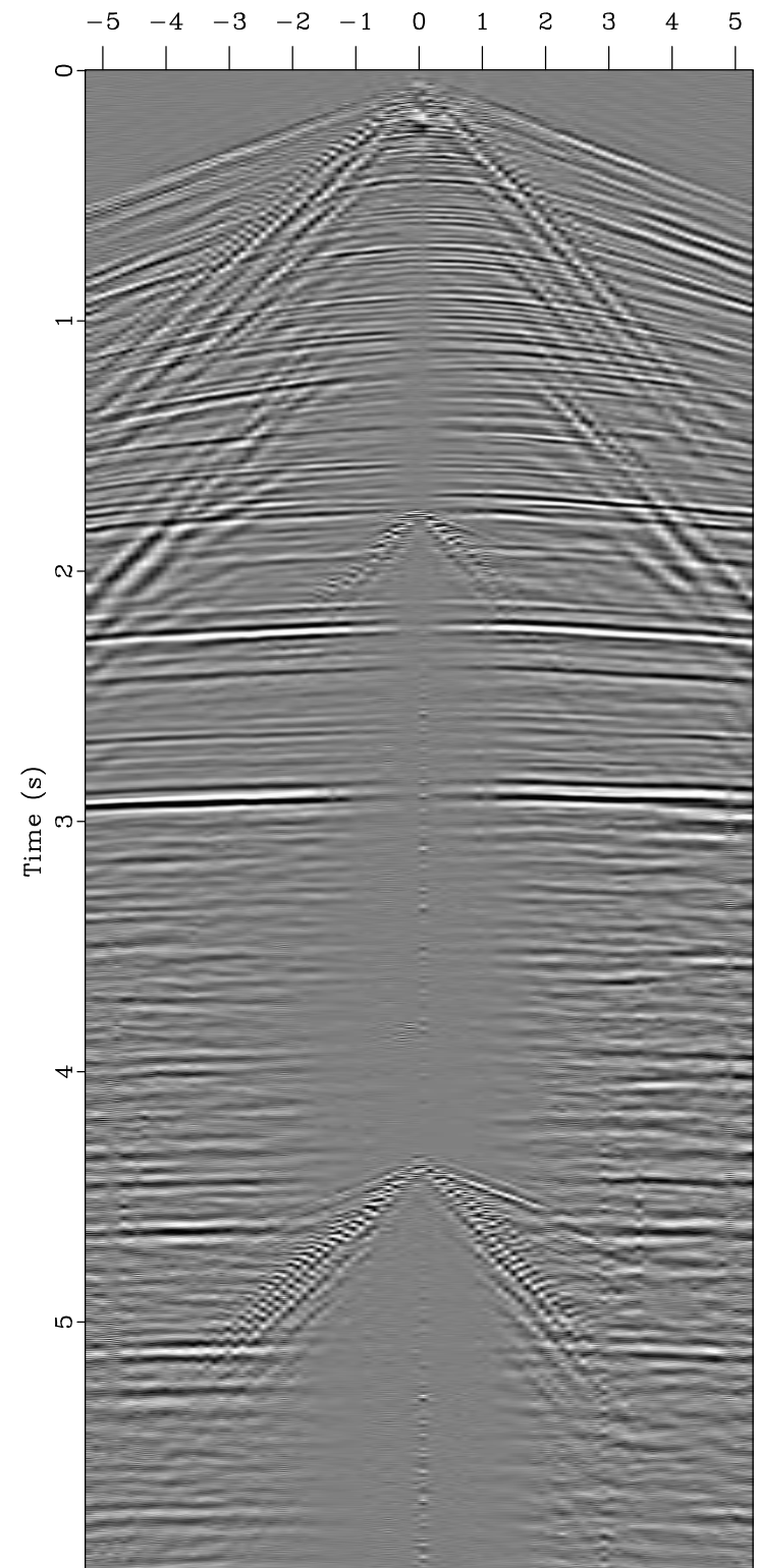
Inverse Radon Transform
