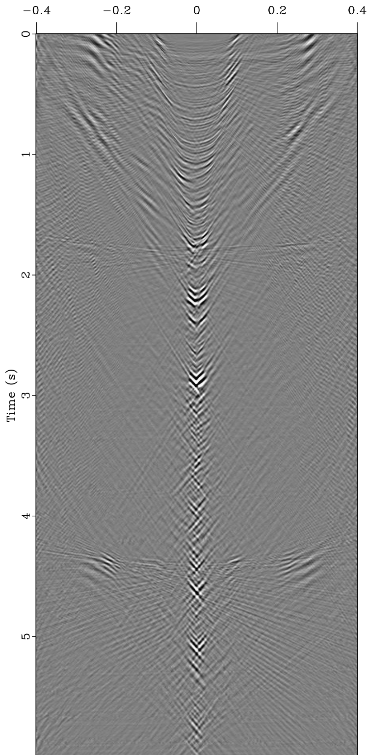
Radon Transform
