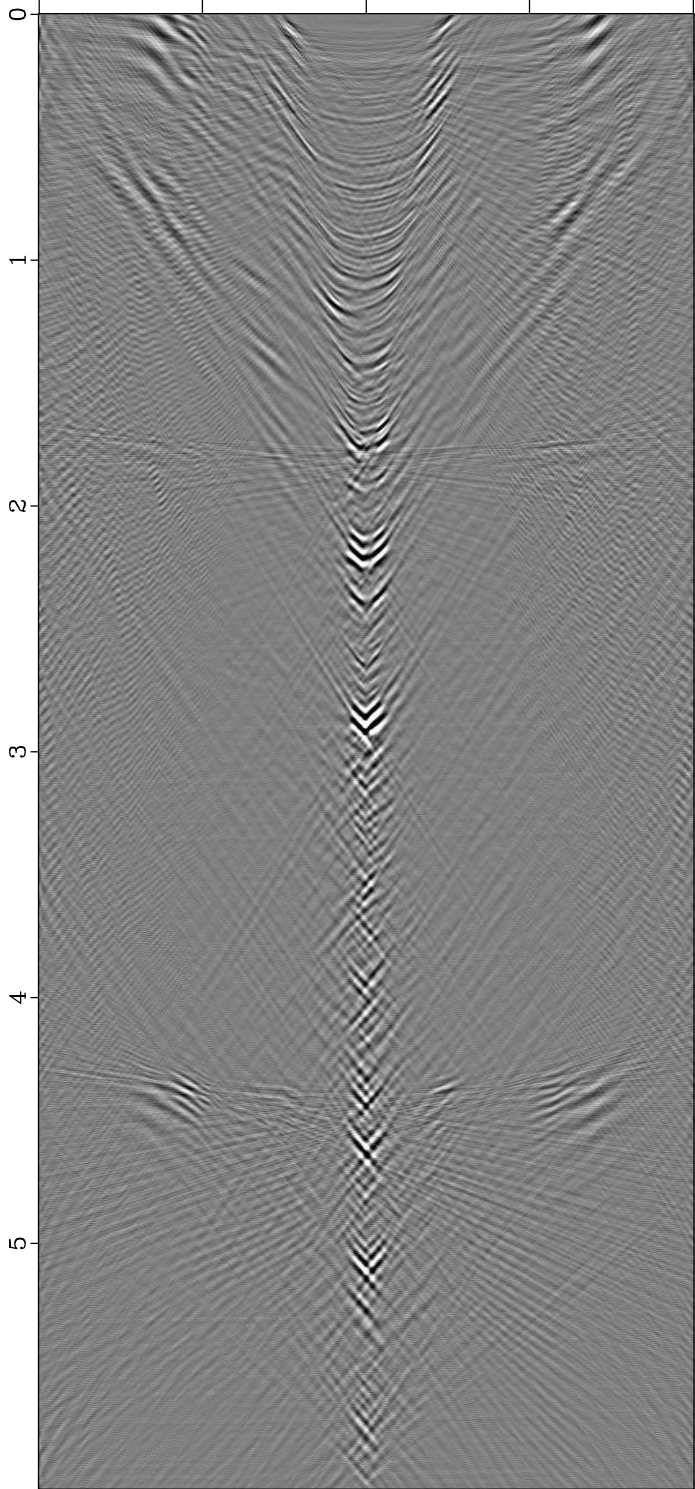
Radon Transform
