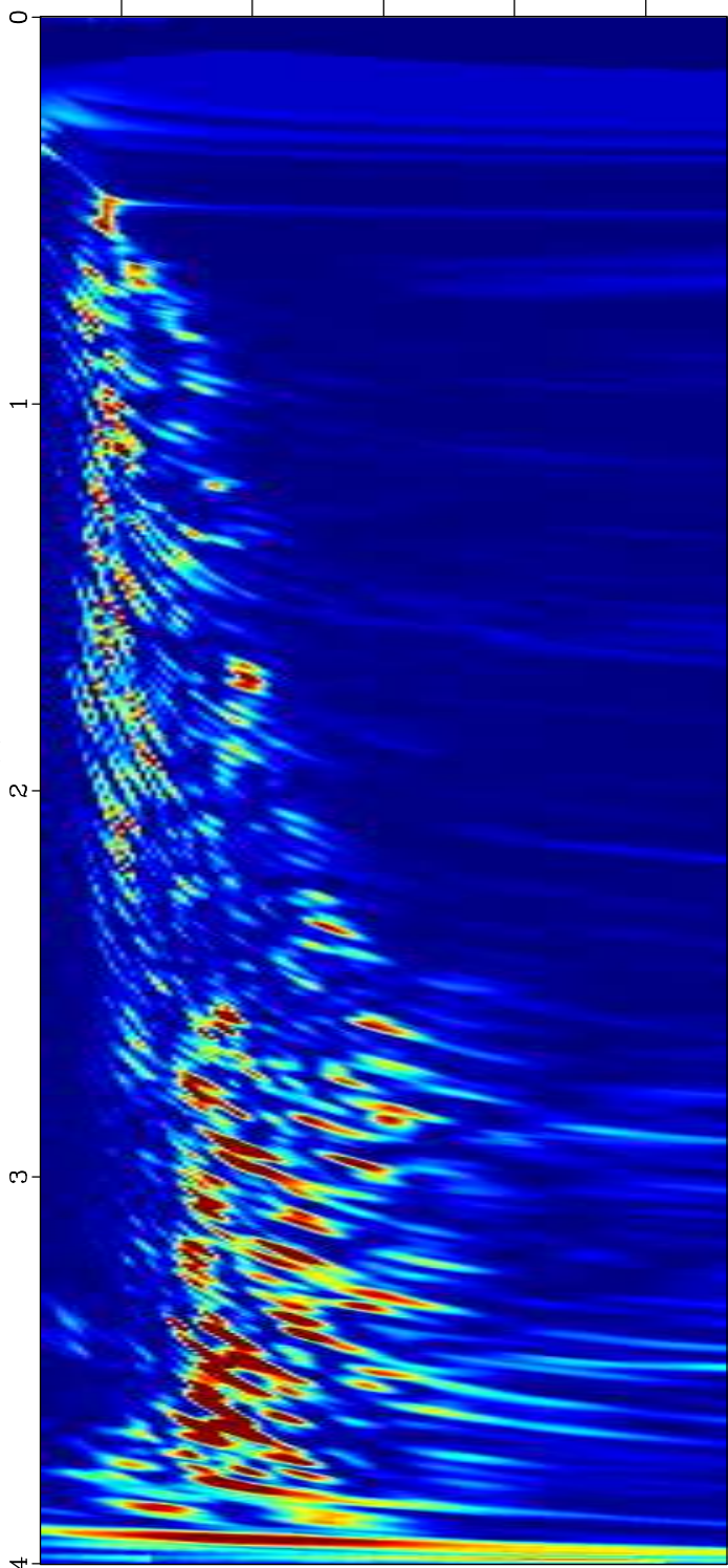
Semblance scan
