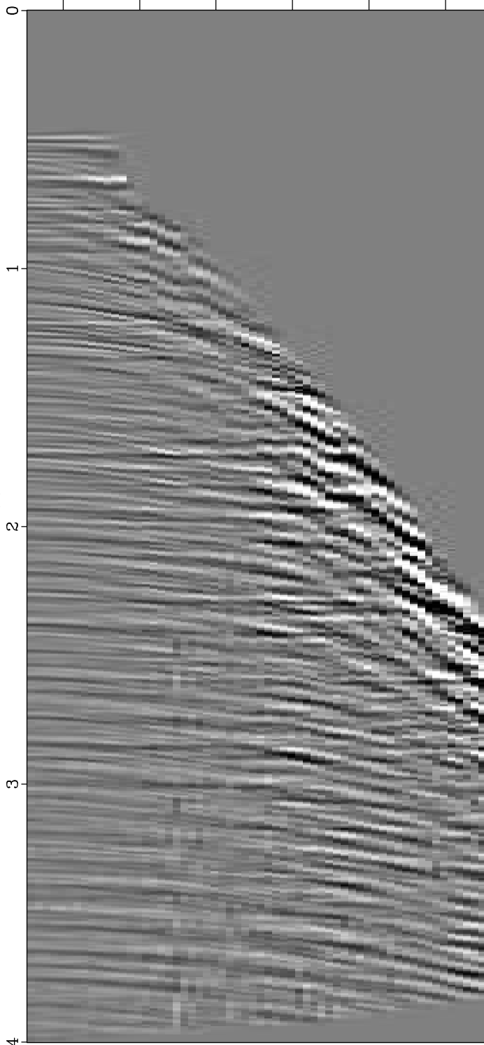
NMO with primary velocity
