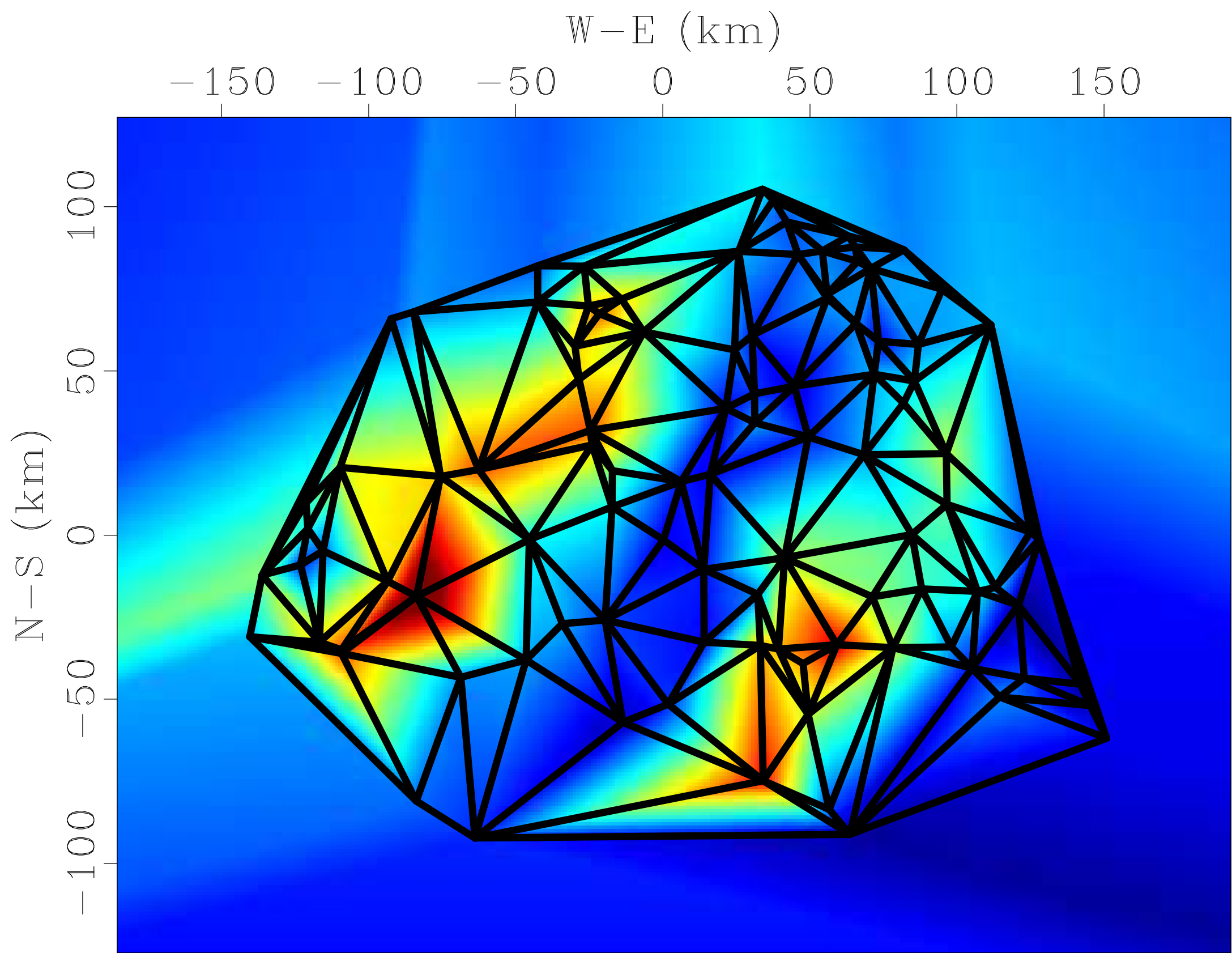
Delaunay Triangulation
