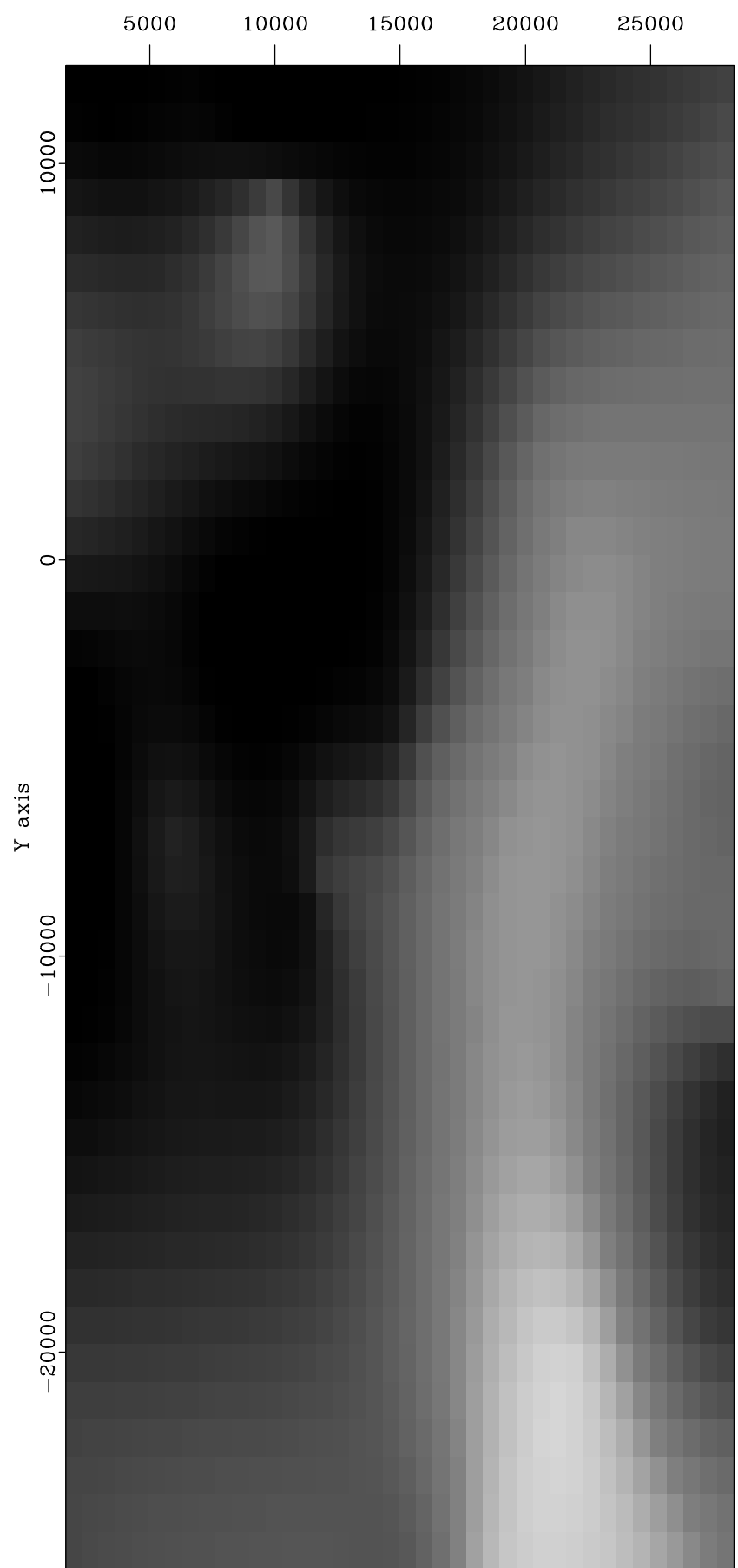
Laplacian Map - Seismic
