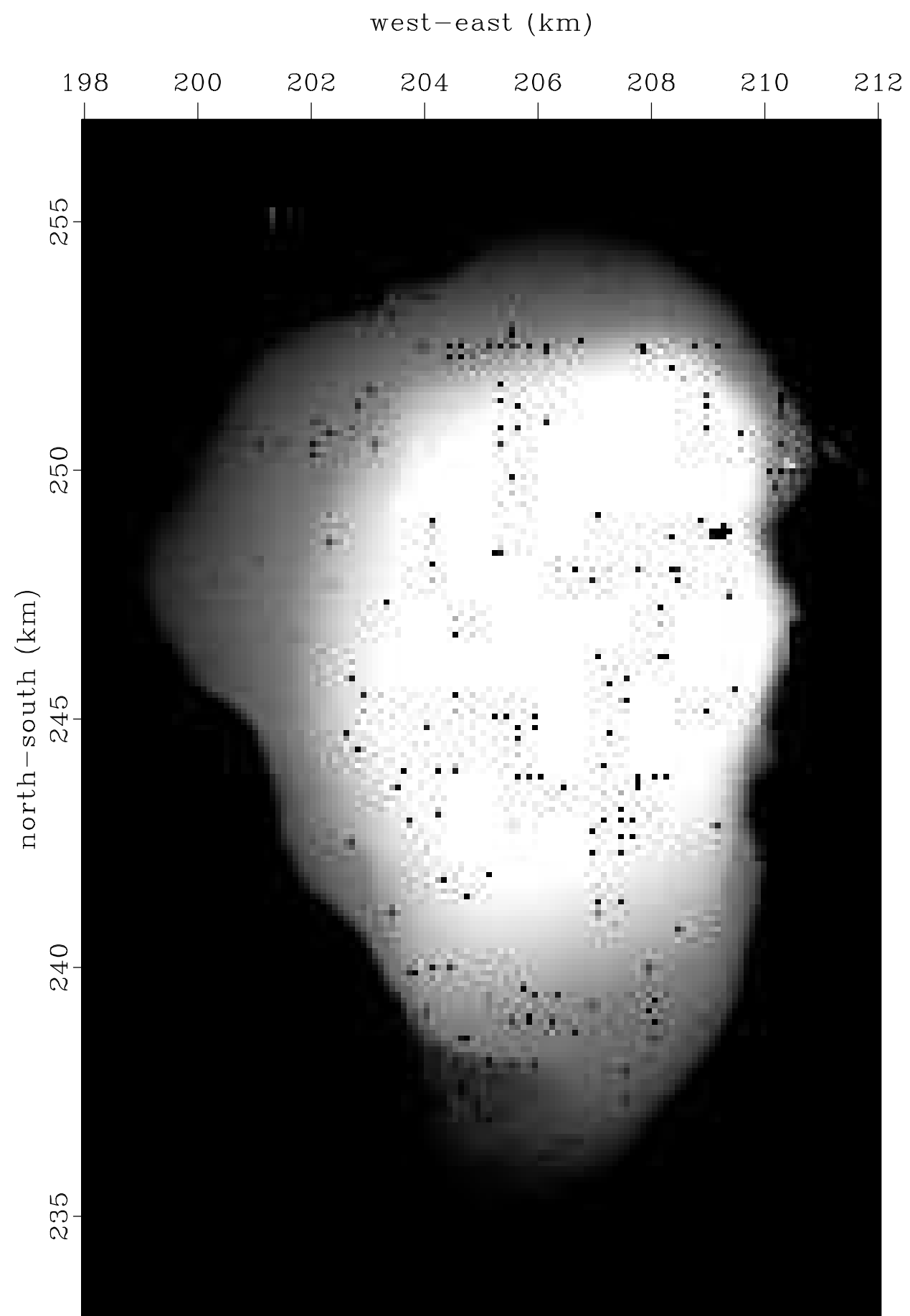
Coarse Binning
