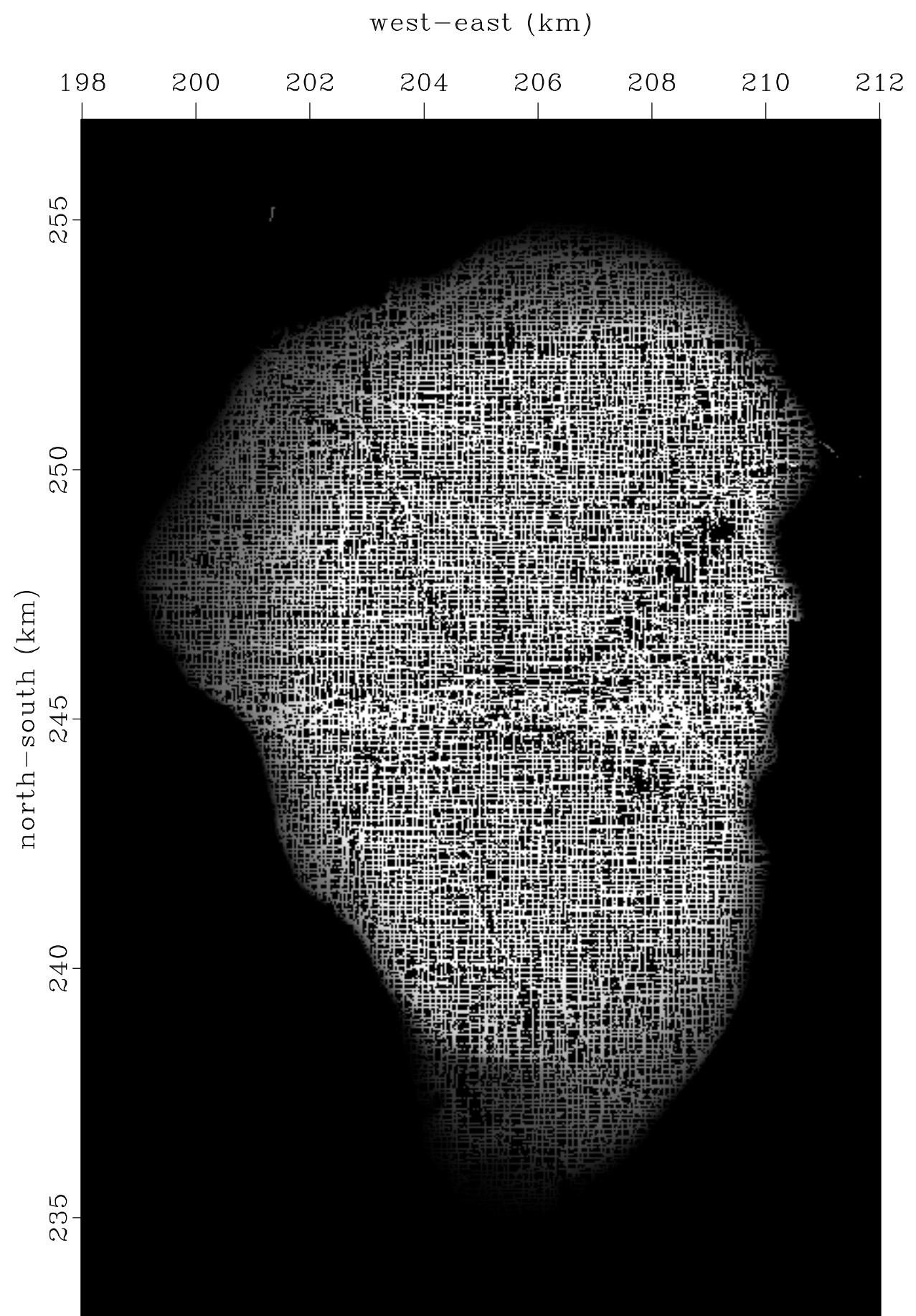
Fine Binning
